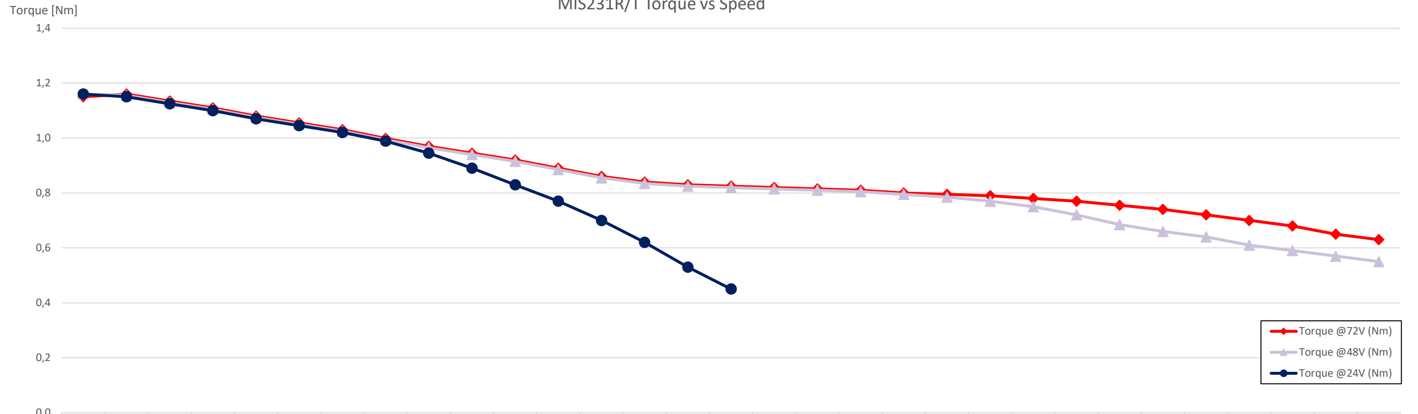
MIS231R/T Torque vs Speed
