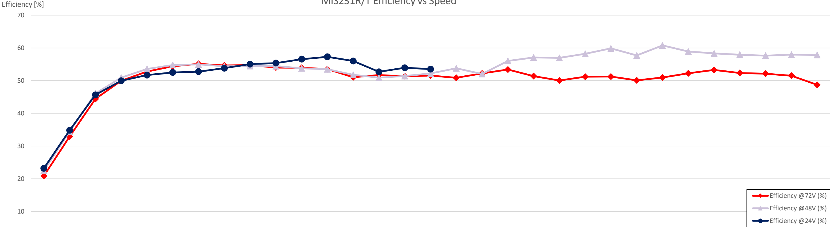
MIS231R/T Efficiency vs Speed
