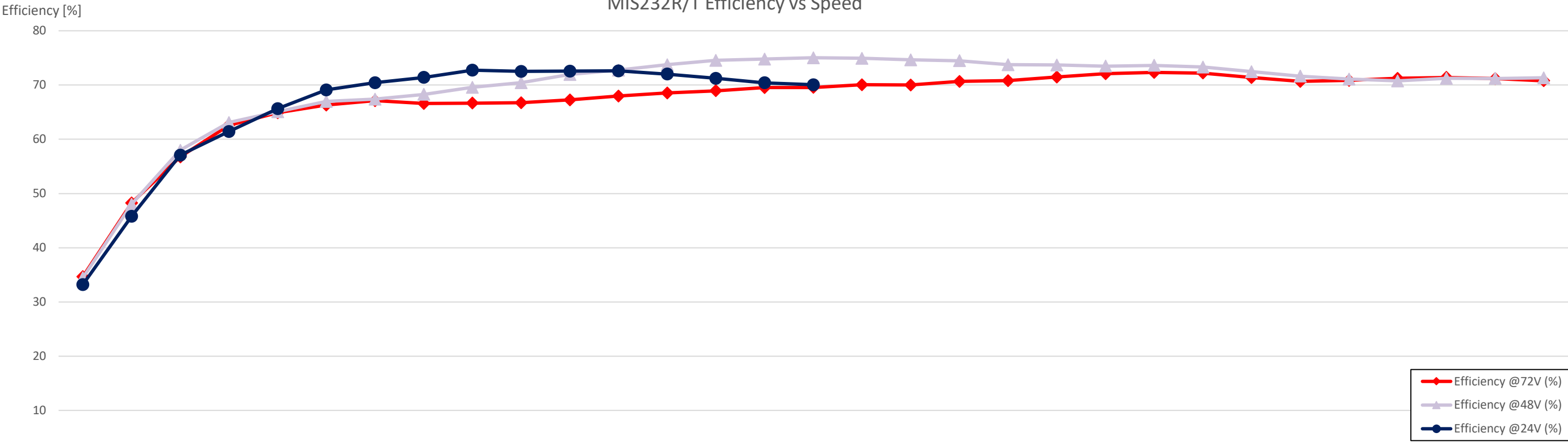
MIS232R/T Efficiency vs Speed
