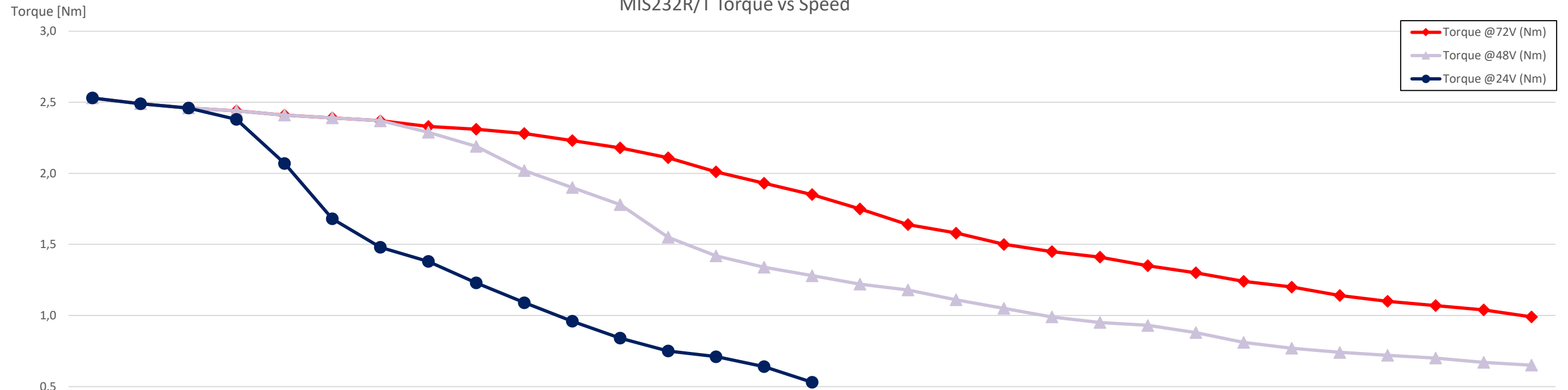
MIS232R/T Torque vs Speed
