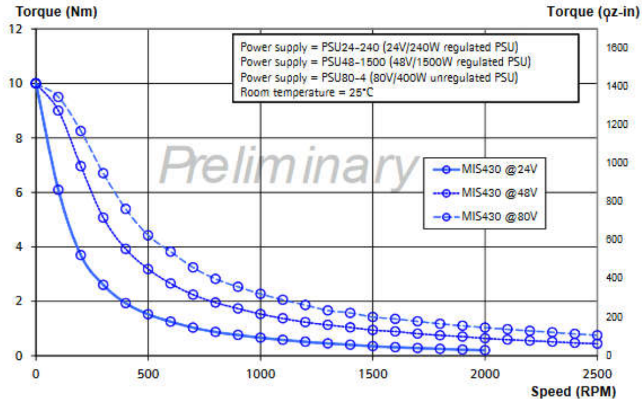
MIS430 motor torque versus speed and supply voltage
