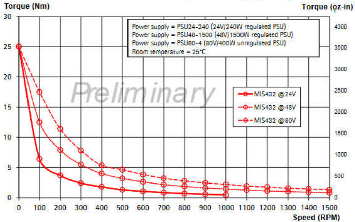
MIS432 motor torque versus speed and supply voltage
